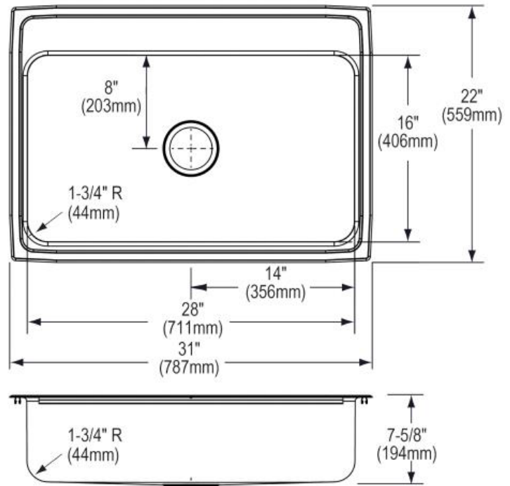
Cutout Dimensions for Drop-in Installation: 30 3/8" x 21 3/8" (772mm x 543mm) with 1 1/2" (38mm) corner radius
